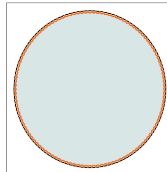
genus 30
