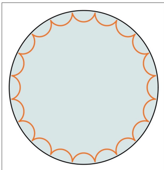
genus 5
