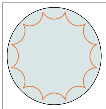
genus 3
