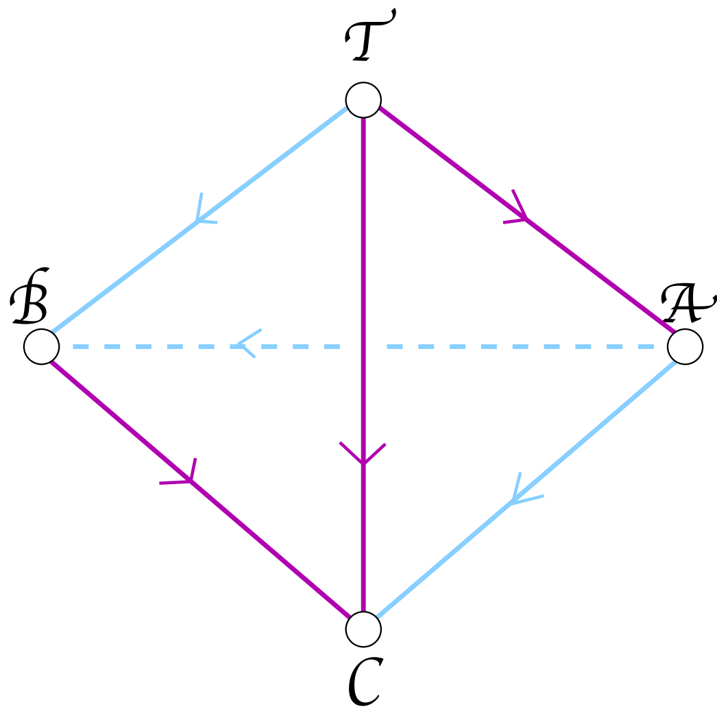
bottom tetrahedron
