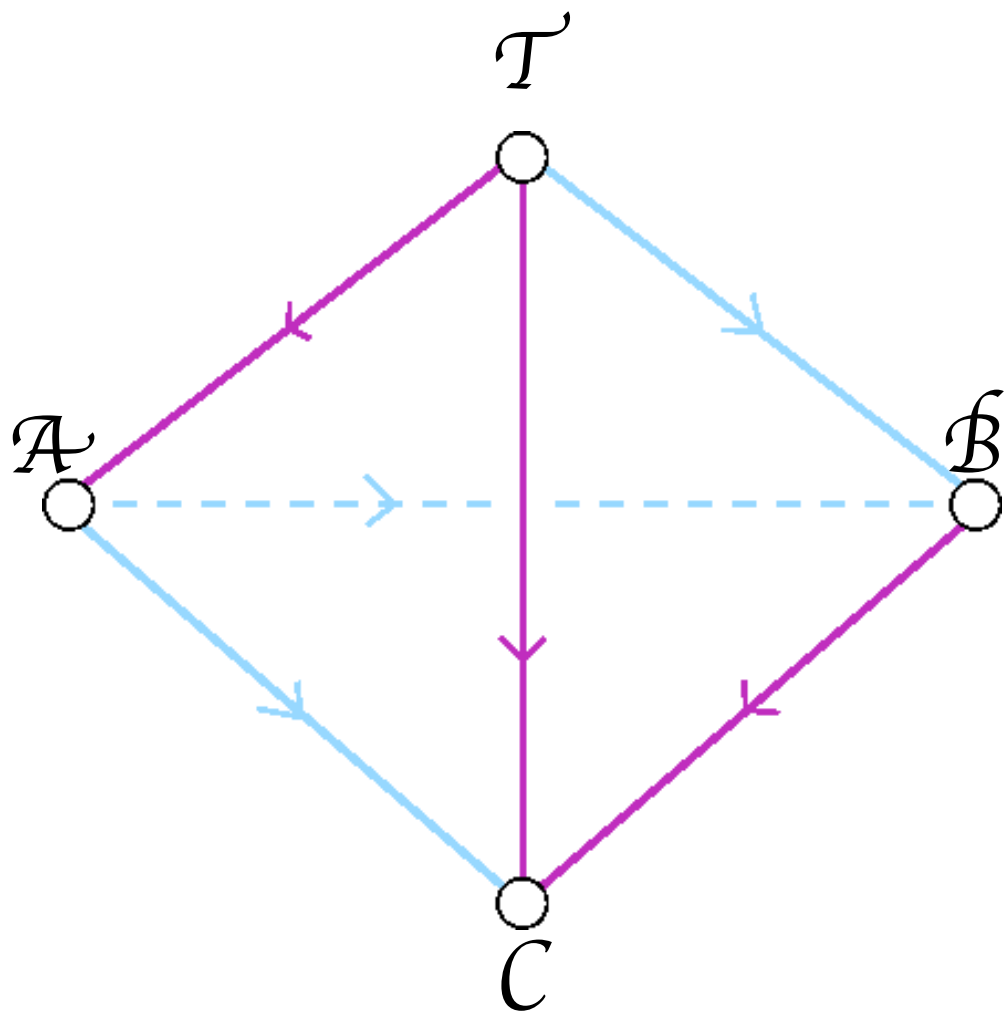
top tetrahedron
