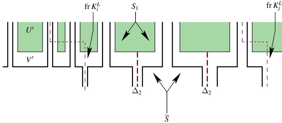
Figure 13: S_1 as a Heegaard surface for W_1 .
