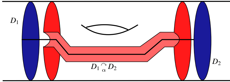
Figure 5: The disc D_1 \frown_{\alpha} D_2
