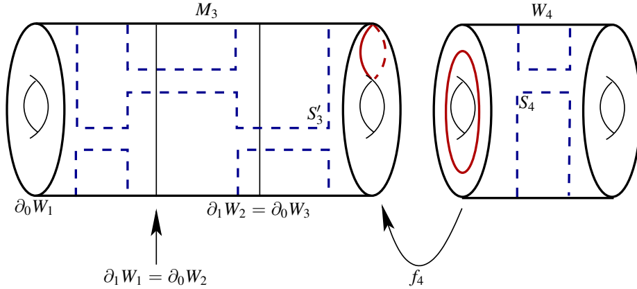
Figure 3: Forming the Heegaard surface S'_4 of M_4
