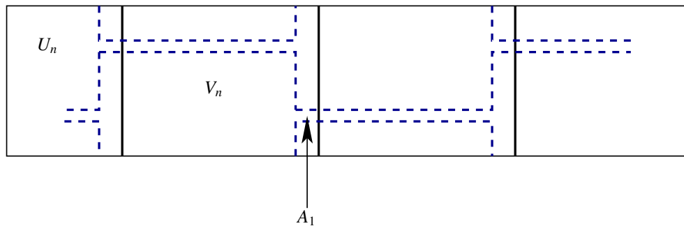
Figure 1: Choosing the splittings of L_i .
