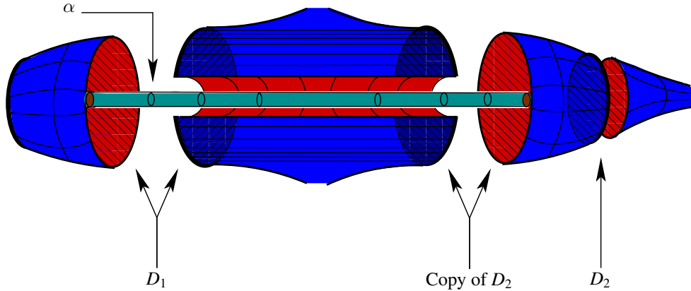
Figure 8: Compressing along \Delta_i
