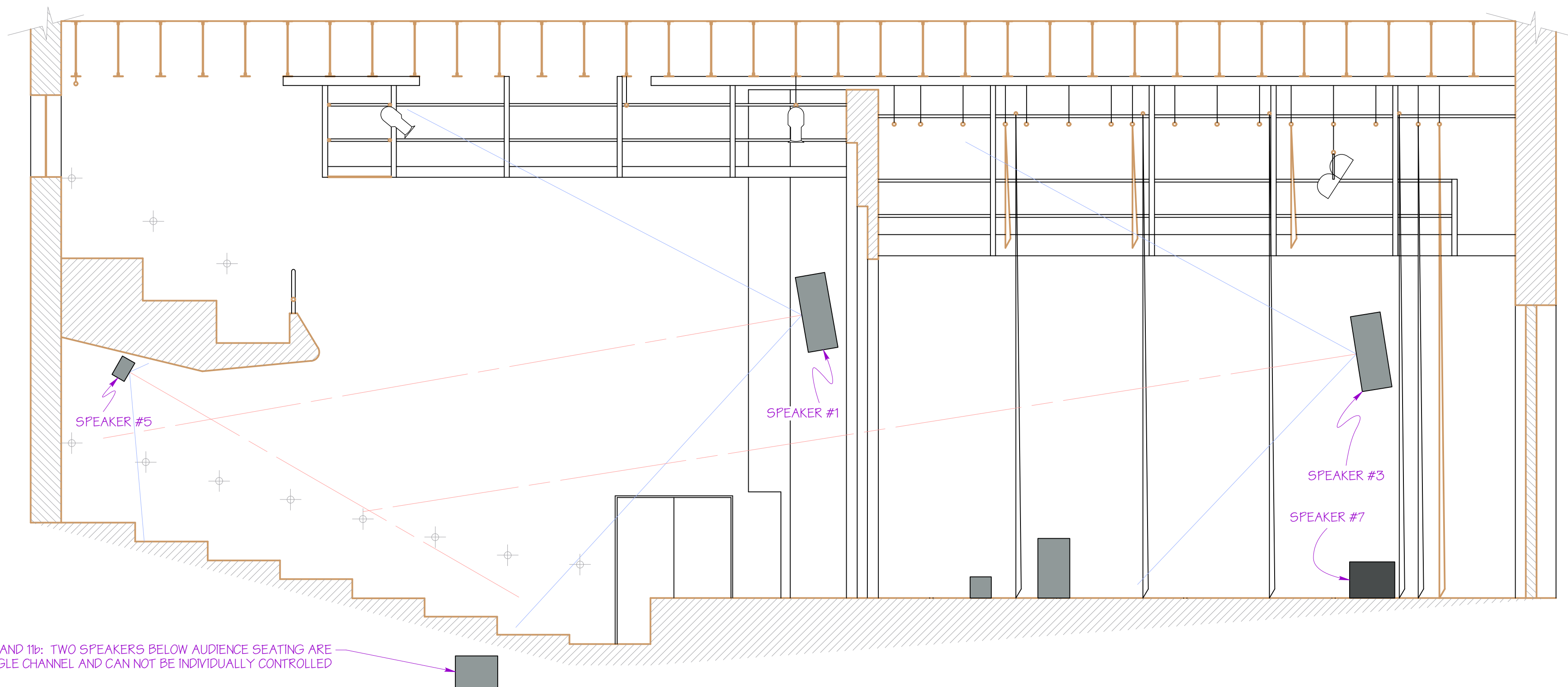
CENTER-LINE SECTION
